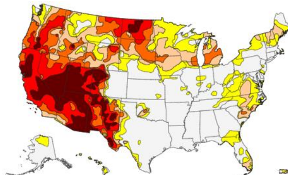
Drought Map as of June 8, 2021
